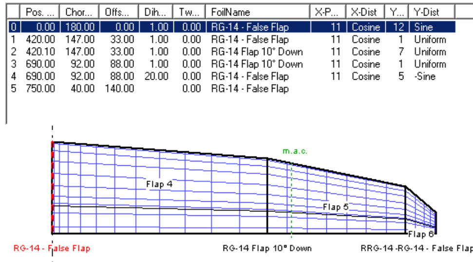
Figure 7: Flap Definition
