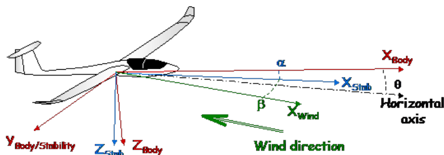
Figure 43: Body and stability axes
