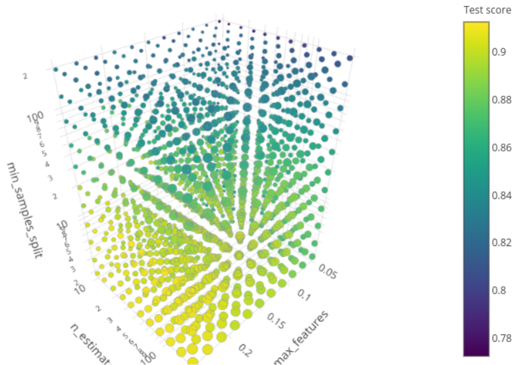
3D visualization of the grid search results
