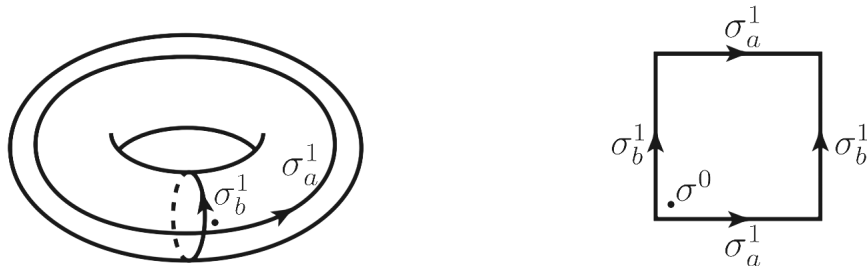
Figure 1.2: CW-complex decomposition of the 2-torus [HAT, p.5]
