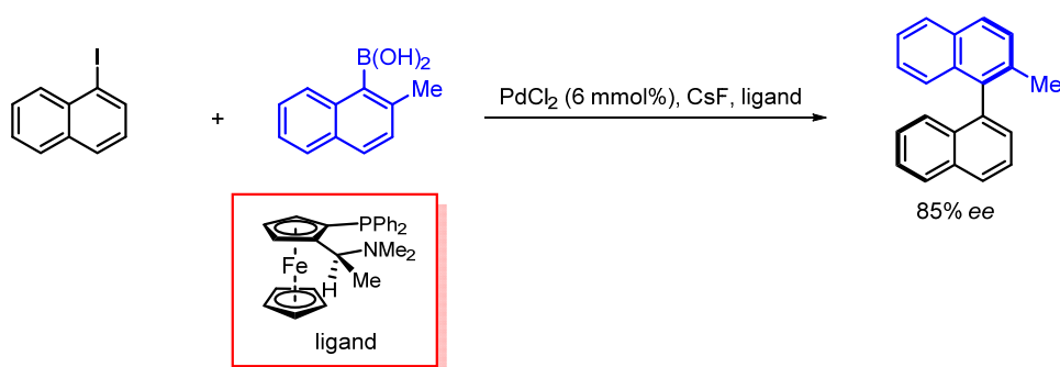
Figure 7. Example of Suzuki enantioselective cross-coupling
